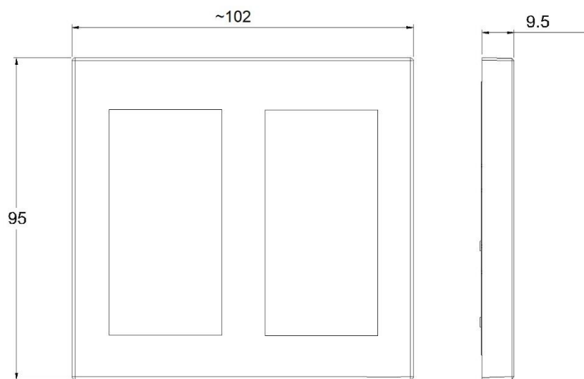
Frame dimensions (in mm)
